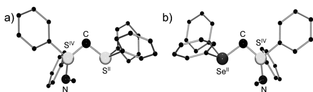
Figure 1. Molecular structures of a) 1 and b) 2 . Ellipsoids are shown at 50% probability. Hydrogen atoms are omitted for clarity. Selected bond lengths [Å] and angles [°]: 1 : S II →C 1.707(2), S IV →C 1.648(2); S II →C←S IV 106.67(14). 2 : Se II →C: 1.876(3), S IV →C 1.654(3); Se II →C←S IV 105.48(17).
